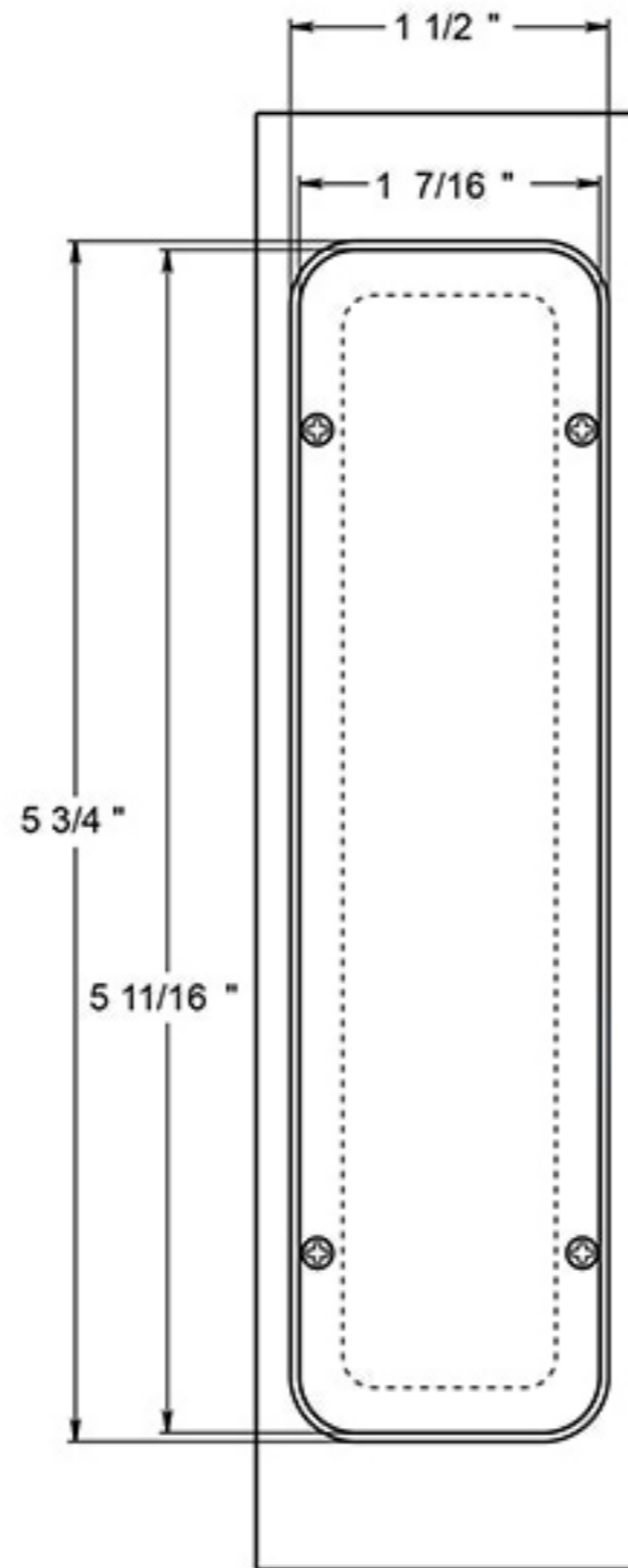
Back View
